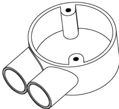
M4 Brass thread Isometric view
