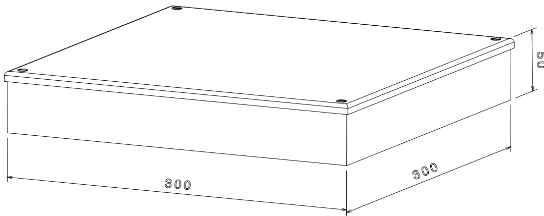
Isometric view
